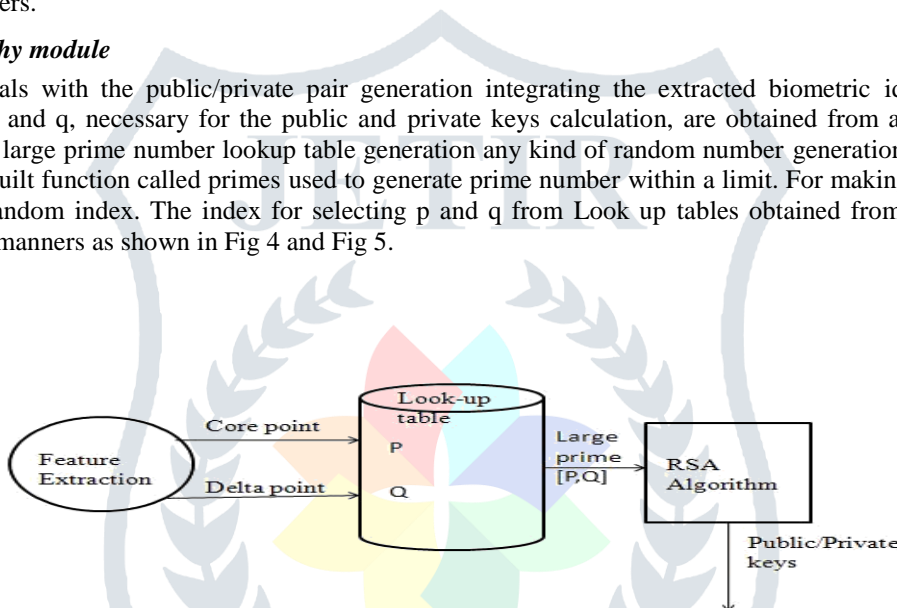
Fig 4.The private/public keys pair generation using Core and Delta point.
