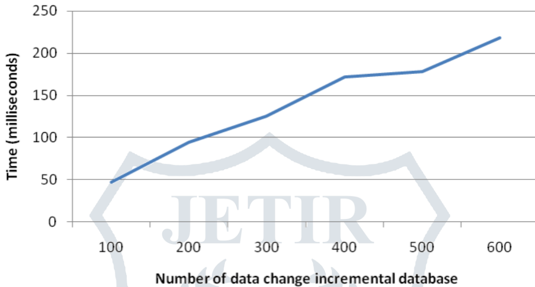
Figure 2: Graph for incremental K-means result[3]
