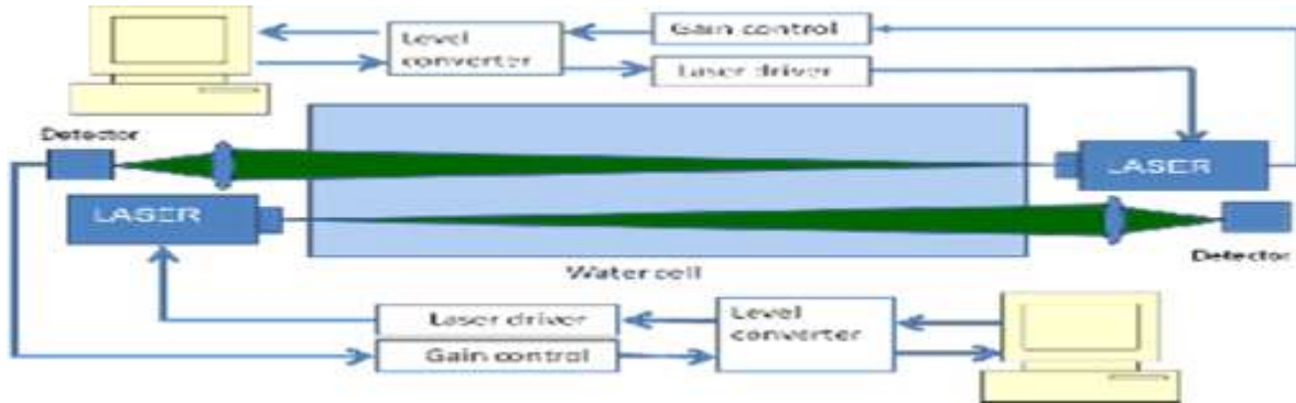
Fig.1 Block diagram of overall system
