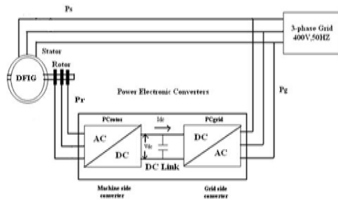
Fig.1. DFIG system with power electronic converters.
