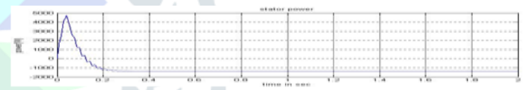
Fig.6. Stator power waveform
