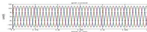
Fig.18. Grid current waveform
