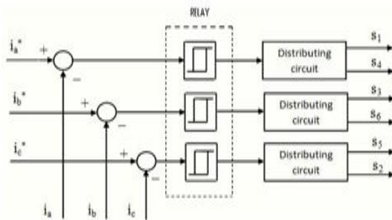
Fig.4. block diagram of current control
