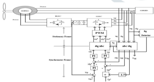
Fig. 3. Block Diagram Of Voltage-Oriented Control. The above equation indicates that there is no need to measure the phase-c grid voltage v_{cg} as shown in fig.3.1. In practice, the grid voltage may contain harmonics and be distorted, so digital filters or phase-locked loops (PLLs) may be used for the detection of grid voltage angle \theta_g .
