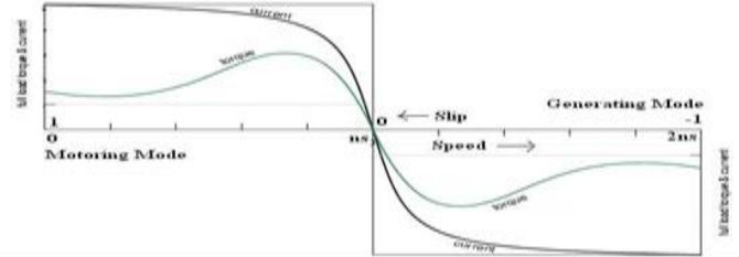
Fig. 2. Torque-Speed characteristics of the DFIG
