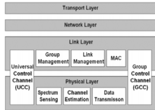
Figure 2 General ISO/OSI Model for Cognitive Radio
