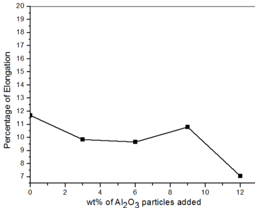
Figure 7: Comparison of percentage of elongation in cast alloy and composites with increasing addition of Al 2 O 3 powder.
