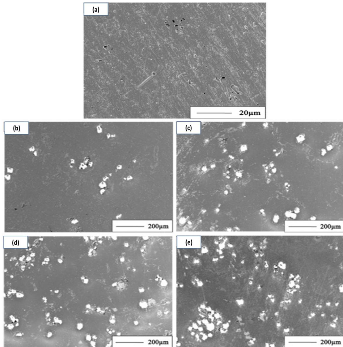
Figure 1: SEM micrographs of (a) cast alloy and different cast composites developed by increasing amounts of \text{Al}_2\text{O}_3 powder designated as (b) AMP3, (c) AMP6, (d) AMP9 and (e) AMP12 respectively.
