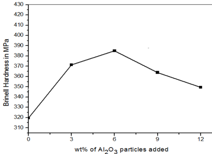
Figure 3: Comparison of hardness in cast alloy and composites developed by increasing addition of Al 2 O 3 powder.
