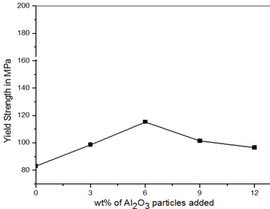
Figure 5: Comparison of yield strength in cast alloy and composites with increasing addition of Al 2 O 3 powder.
