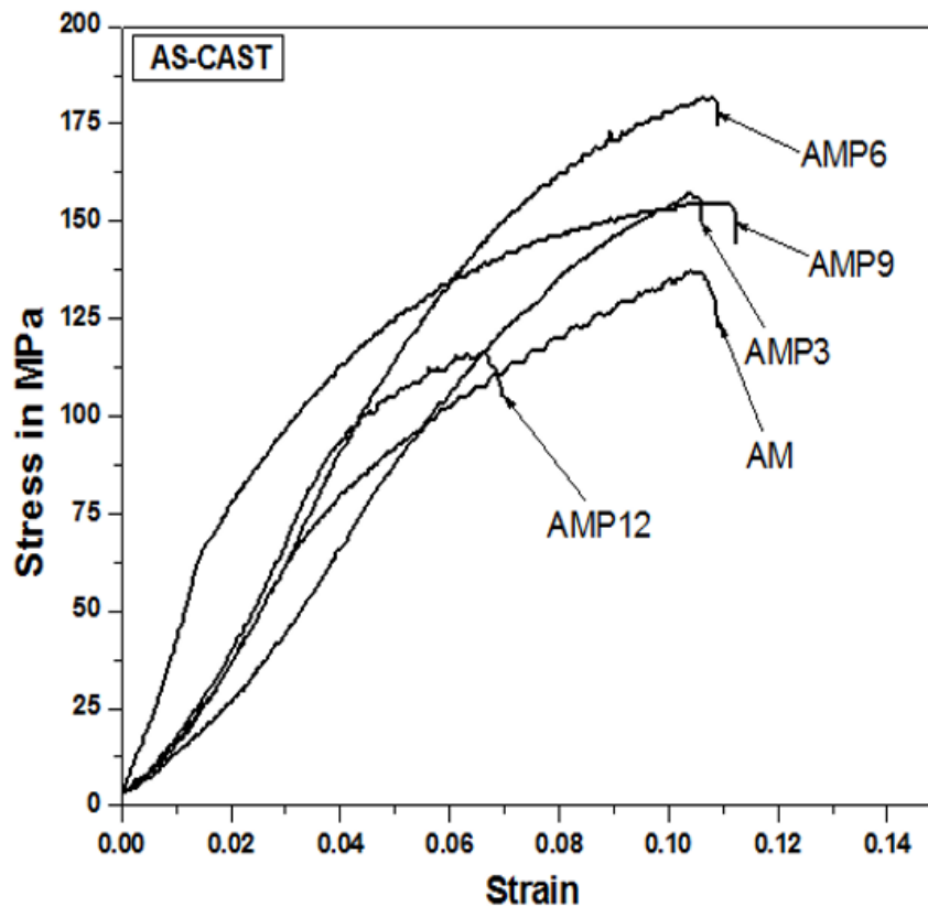
Figure 4: Tensile stress-strain behaviour of cast alloy and composites developed by addition of 0, 3, 6, 9 and 12 wt% of Al 2 O 3 powder.
