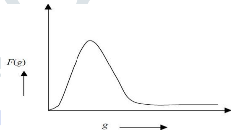
Fig. 4: Gamma distribution
