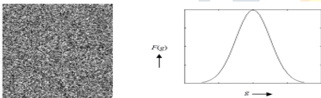
Figure 1: (a) Gaussian noise (mean=0, variance 0.05), (b) Gaussian distribution
