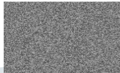
Fig. 3: Speckle noise
