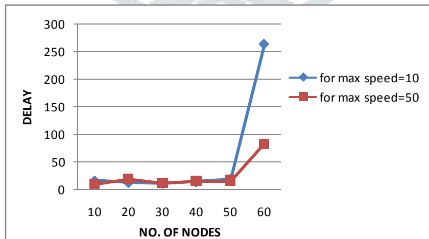
Figure 1.1 shows no. of nodes vs delay graph for different maximum speed.
