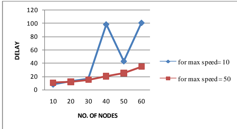
Figure 1.3 shows no. of nodes vs delay graph for different max speed in low mobility.
