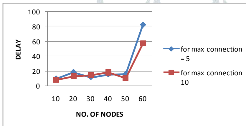
Figure 1.2 shows no. of nodes vs delay graph for different no. of connections in high mobility.
