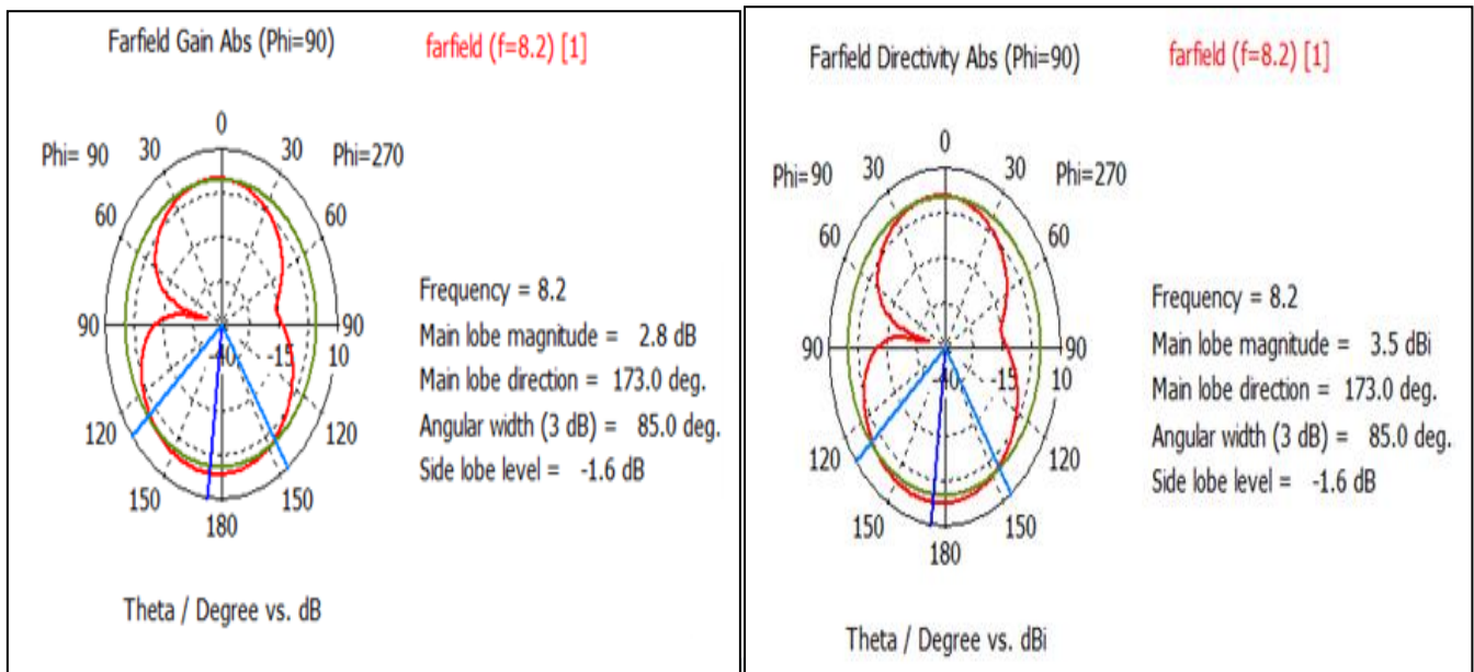
2D Radiation pattern plot for - Fig. 2(c) Gain=2.8 dB
