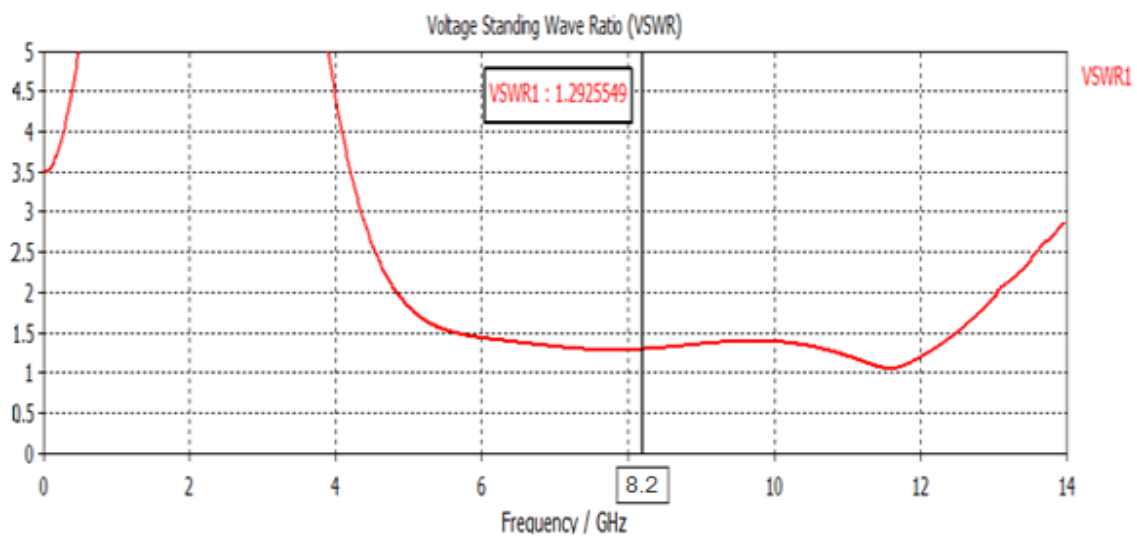
Fig. 2(b) VSWR versus Frequency Plot, VSWR =1.29
