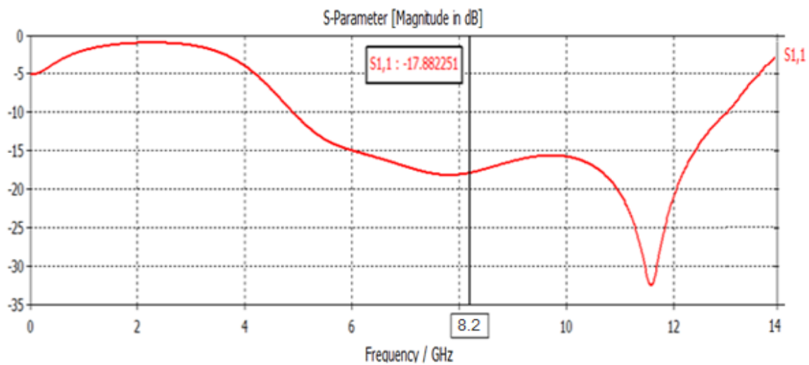
Fig. 2(a) Return Loss versus Frequency Plot, Return Loss = -17.88 dB
