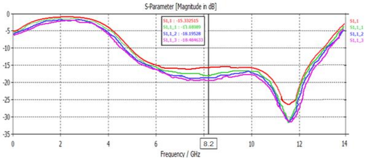
Fig. 3 Return Loss versus Frequency Plot for Various values of Substrate Thickness (Red Line for h = 1.4mm, Green Line for h = 1.58mm, Blue Line for h = 1.65mm, Purple Line for h = 1.7mm)
