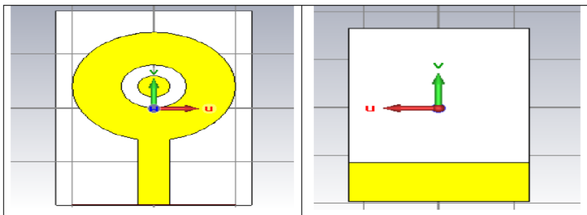
Fig. 1 Front and back view of Circular Microstrip Patch Antenna with circular slot.
