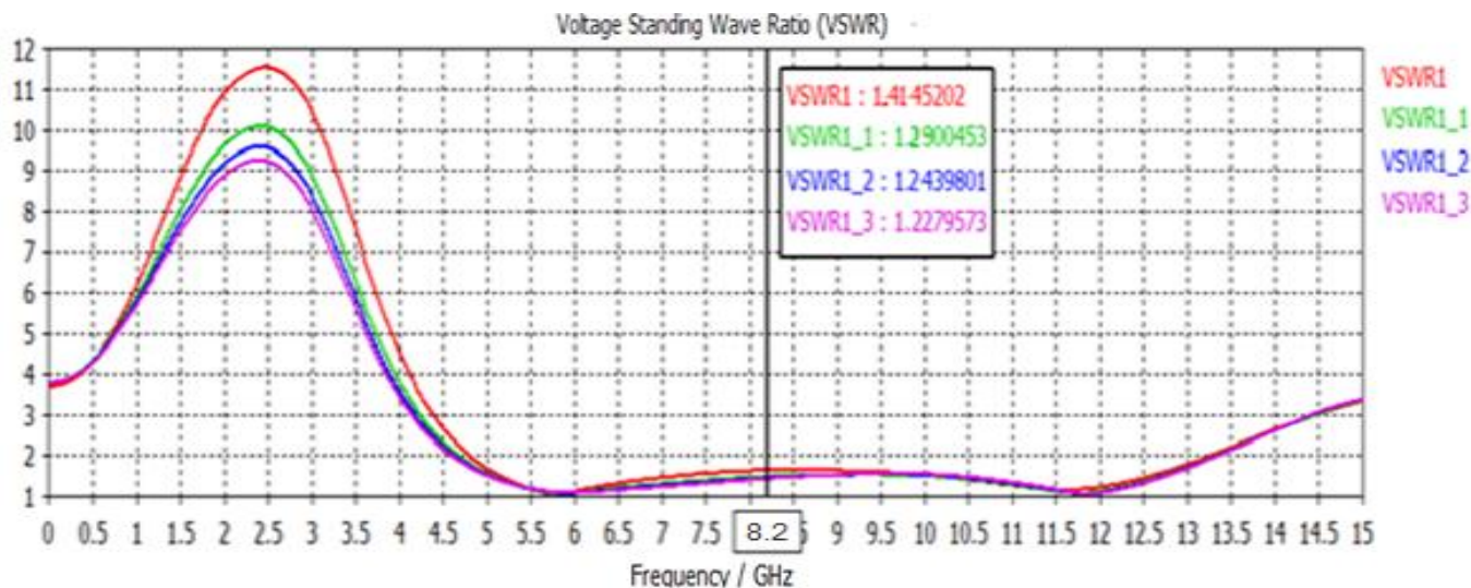
Fig. 4 VSWR versus Frequency Plot for Various values of Substrate Thickness (Red Line for h = 1.4\text{mm} , Green Line for h = 1.58\text{mm} , Blue Line for h = 1.65\text{mm} , Purple Line for h = 1.7\text{mm} )
