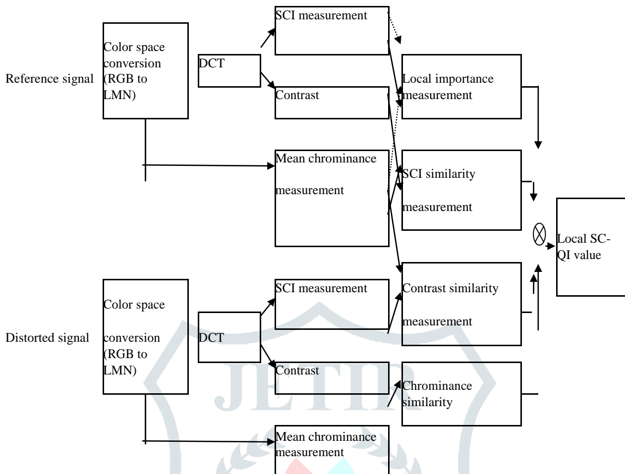
Fig.1. Block diagram for measurement of quality for full-reference image.
