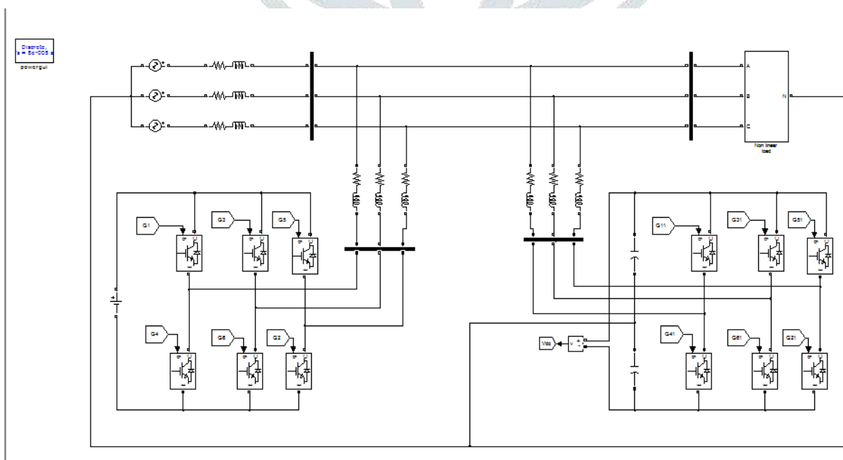
Fig.2. MATLAB Simlink model
