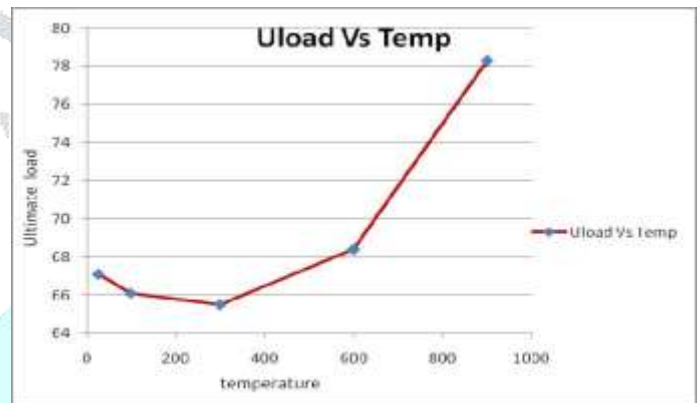
Fig 4.1 Unload vs Temp Curve
