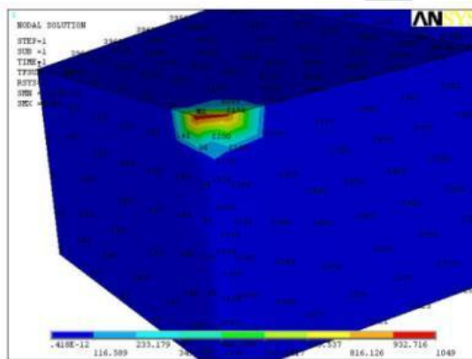
Fig 6: nodal temperature distribution of cutting tool
