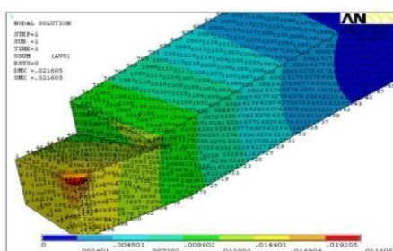
Fig 4: Deformation of cutting tool.
