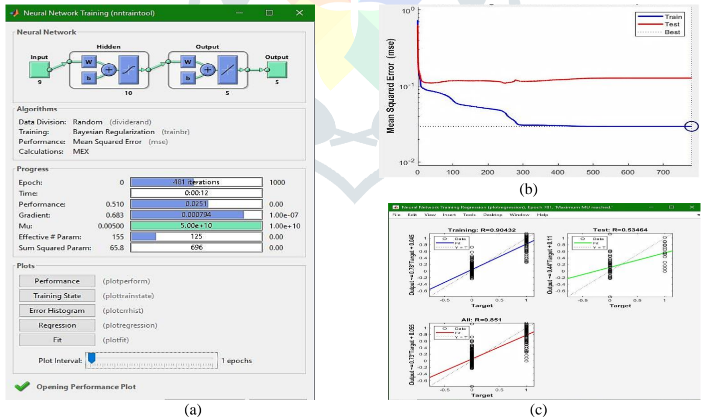
Fig.3 Output screens from MATLAB runs (a) BRANN model (b) performance (c) Regression.
