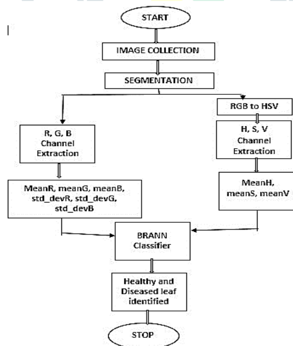
Fig.2 Flow chart of Rice Leaf Disease Identification.
