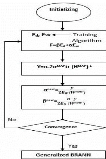
Fig.2 Flow Chart of BRANN Algorithm.
