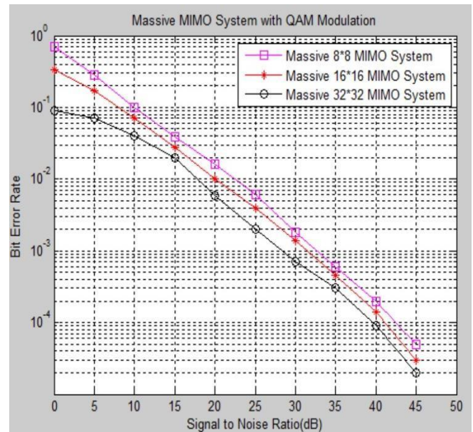
Figure 8: BER vs SNR for Matched Filter Detection Spectrum Sensing Different System
