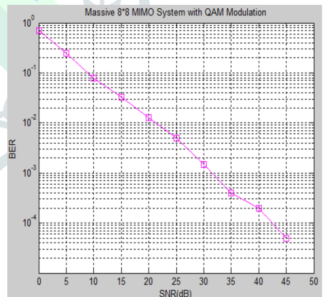
Figure 5: BER vs SNR for Matched Filter Detection Spectrum Sensing 8×8 System
