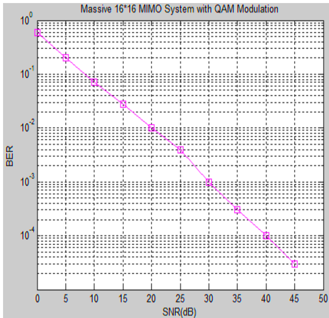
Figure 6: BER vs SNR for Matched Filter Detection Spectrum Sensing 16x16 System
