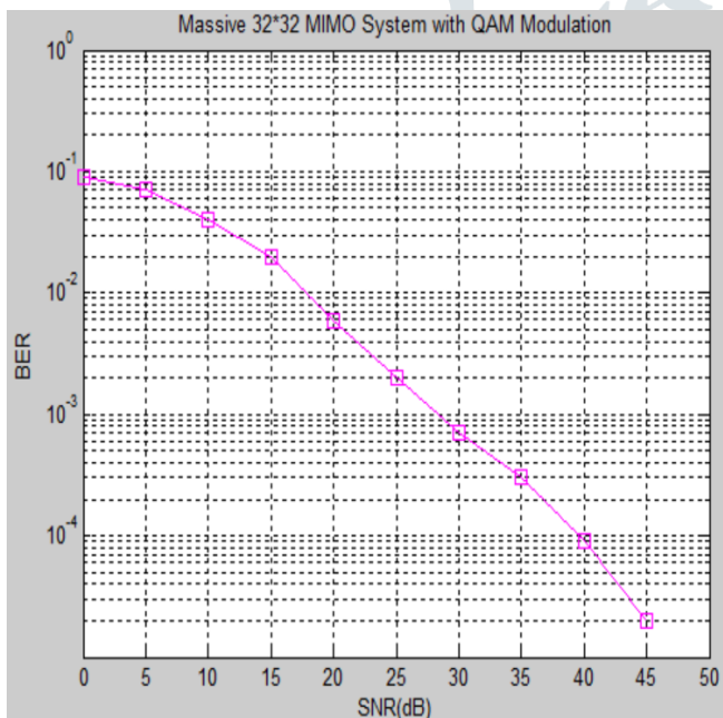
Figure 7: BER vs SNR for Matched Filter Detection Spectrum Sensing 32x32 System
