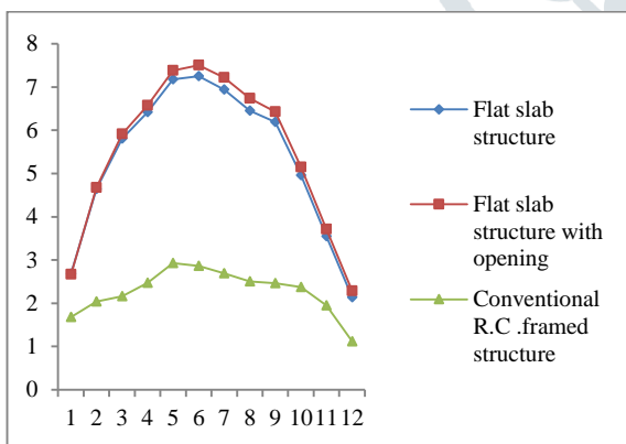
Figure 3.Linear Static Analysis.
