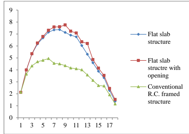
Figure 6. Linear Dynamic Analysis
