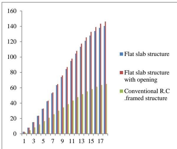
Figure11. Linear Static Analysis.
