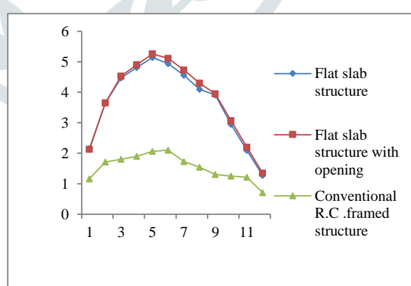
Figure 4.Linear Dynamic Analysis
