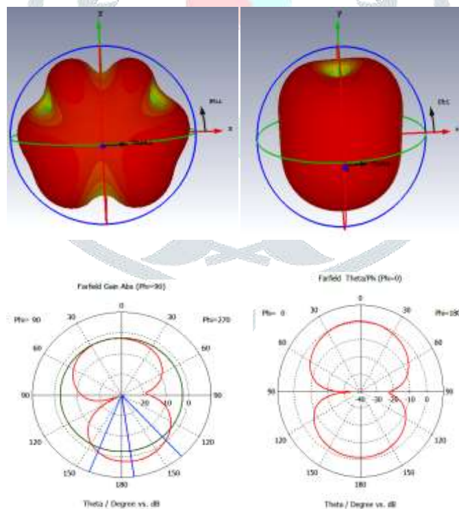
Figure 12: Radiation pattern
