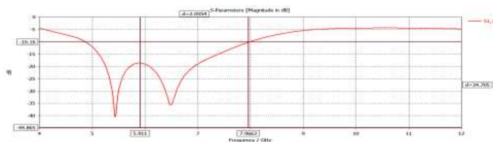
Figure 9: Bandwidth
