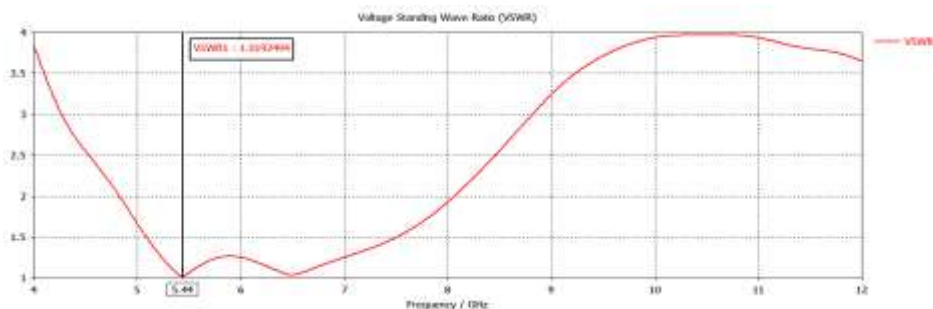
Figure 7: VSWR
