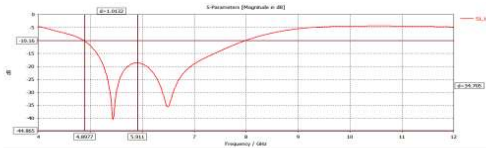
Figure 6: Bandwidth
