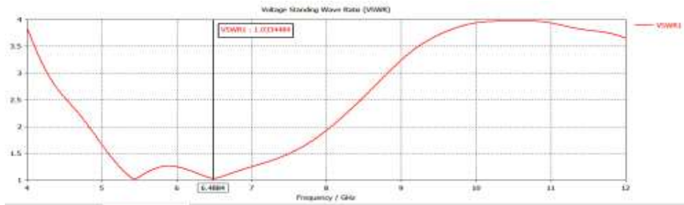
Figure 10: VSWR
