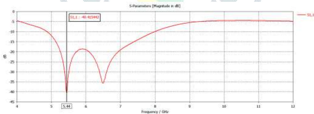
Figure 5: Return loss
