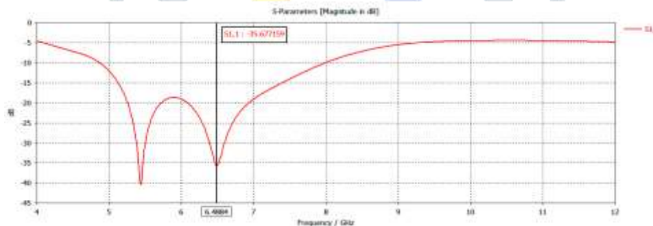
Figure 8: Return loss
