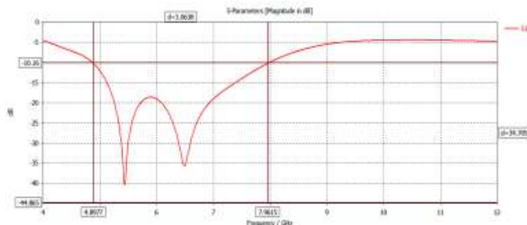
Figure 11: Bandwidth
