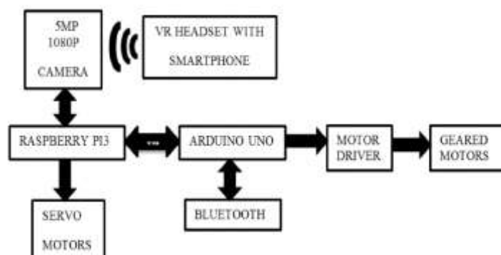
Fig 1: Telepresence surveillance robot
