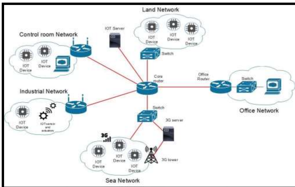
Fig.1: smart-company network topology
