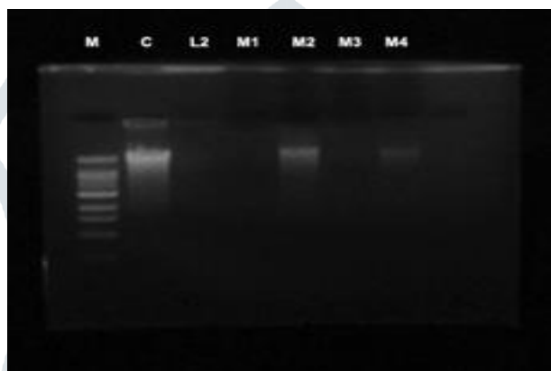
Fig 3 : DNA cleavage: M: Standard DNA, C: Control DNA (untreated pBR 322)L2:Ligand(L),M1:Cu(II) complex,M2:Co(II) complex,M3:Ni(II) complex and M4:Zn(II) complex.
