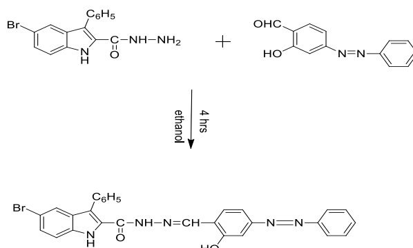
Scheme 1: Synthesis of ligand.
