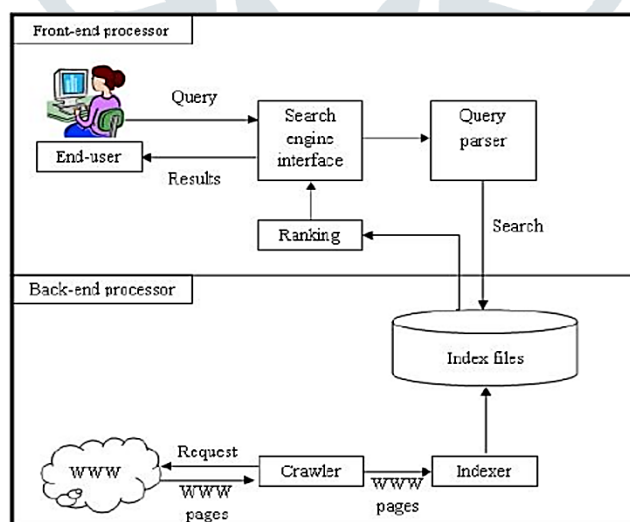
Search Engine Architecture
