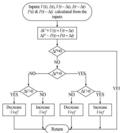
Fig.2. MPPT control algorithm
