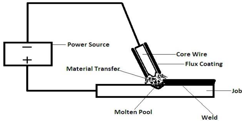
Figure 2: Representation of SMAW set-up.
