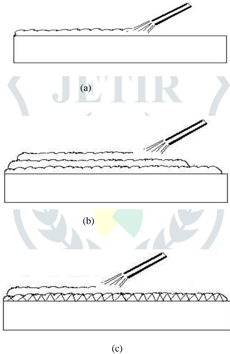
Figure 1: Layout of hardfacing. Hardfacing materials can be added to base metal as a) a single layer, b) certain layers. And sometimes, c) a buffer layer is pasted onto the base metal before the application of hardfacing alloy to provide better bonding between different layers.
