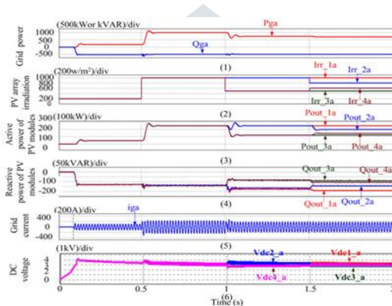
Fig. 6. Simulation results of PV system with traditional active and reactive power control in phase a. (a) Power distribution.
