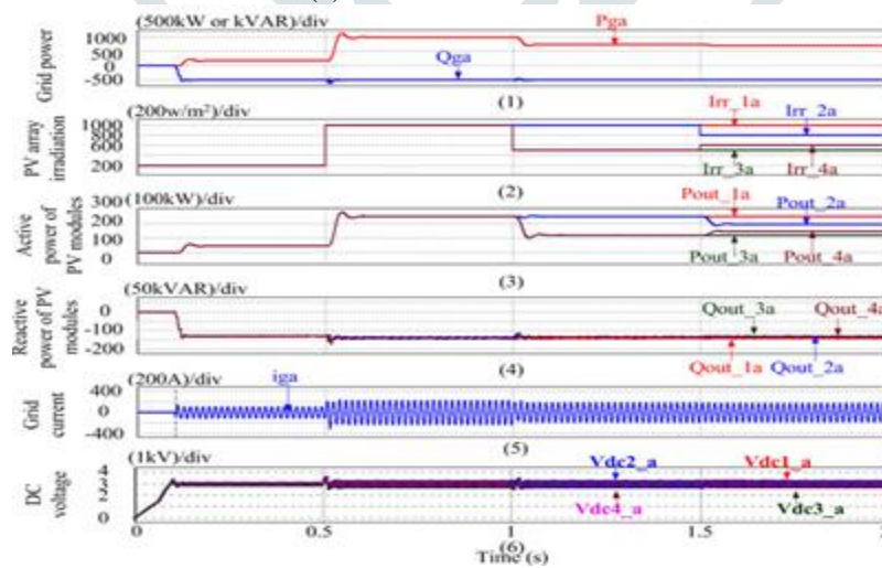
Fig:7. Simulation results of PV system with decoupled active and reactive power with fuzzy control in phase a. (a) Power distribution. (b) Zoomed waveforms at 1.5 s.
