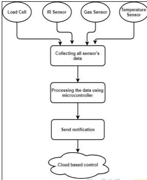
Figure 1 : Process flow diagram for Refrigerator for Monitoring Stored Food Materials
