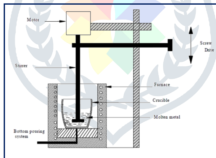
Figure 1: Stir casting method
