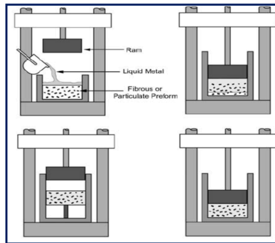
Figure 2: Squeeze casting or pressure infiltration process
