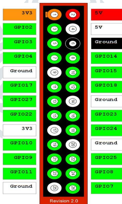
Fig.4 Pin description of Raspberry pi
