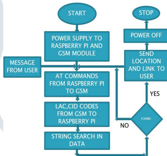
Fig.2 Flow Chart of Location Reporting System
