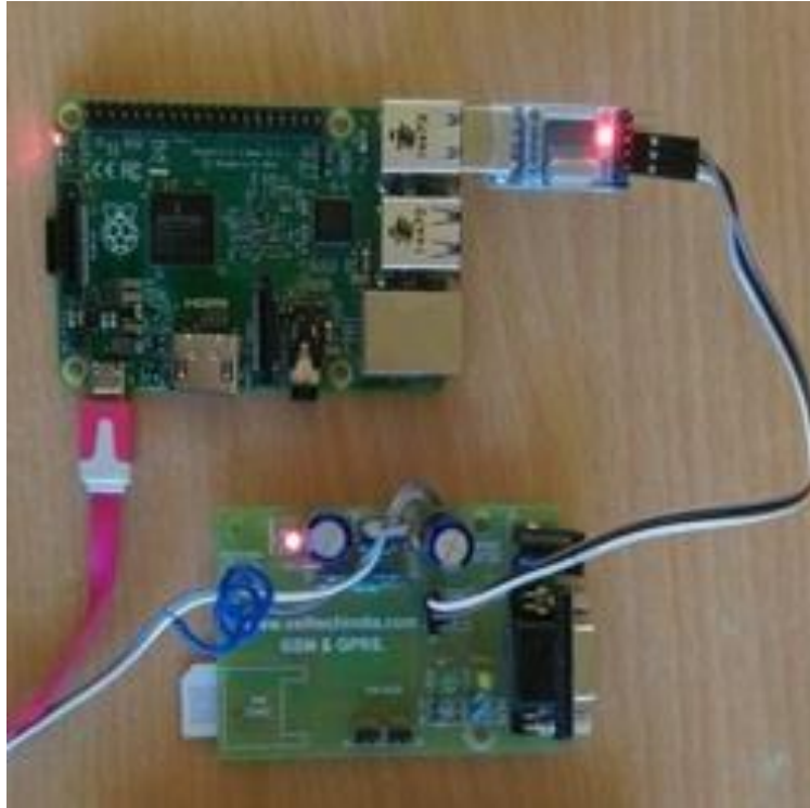
Fig.6 working prototype of location reporting system
