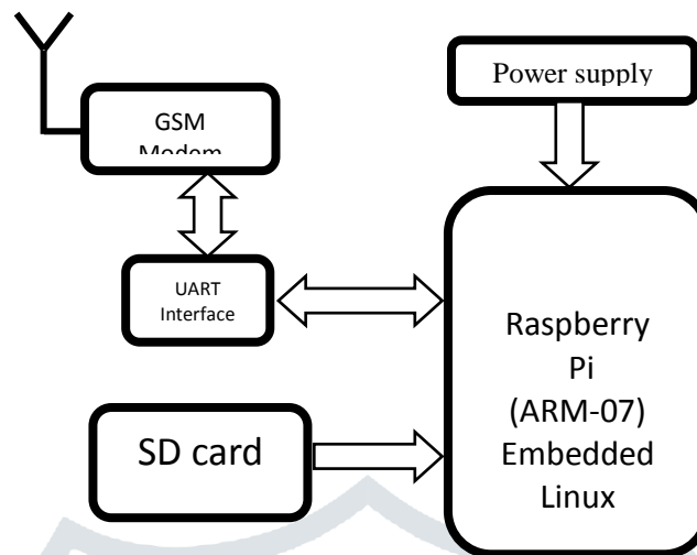
Fig.1 Block Diagram of Location Reporting System
