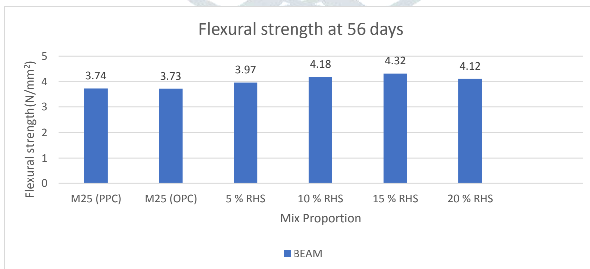
Chart-8 56 days Flexural Strength(Beam)
