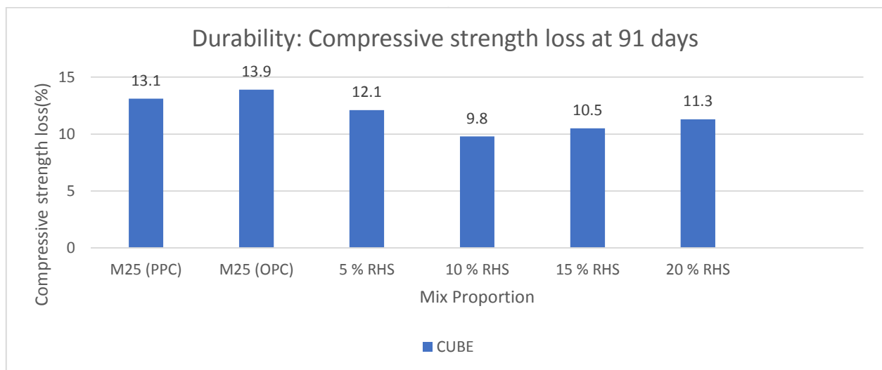
Chart-10 Durability: Compressive strength loss at 91 days
