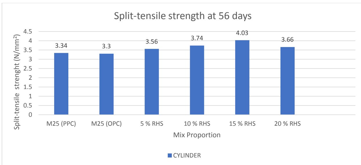
Chart-7 56day split tensile strength(Cylinder)
