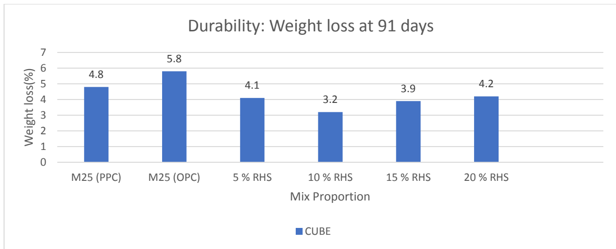
Chart-9 Durability: Weight loss at 91 days
