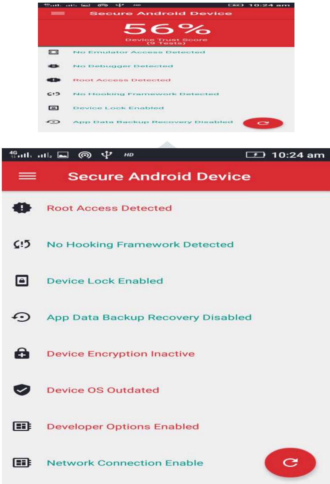
Figure 2: Check how many percent secure our android device.
