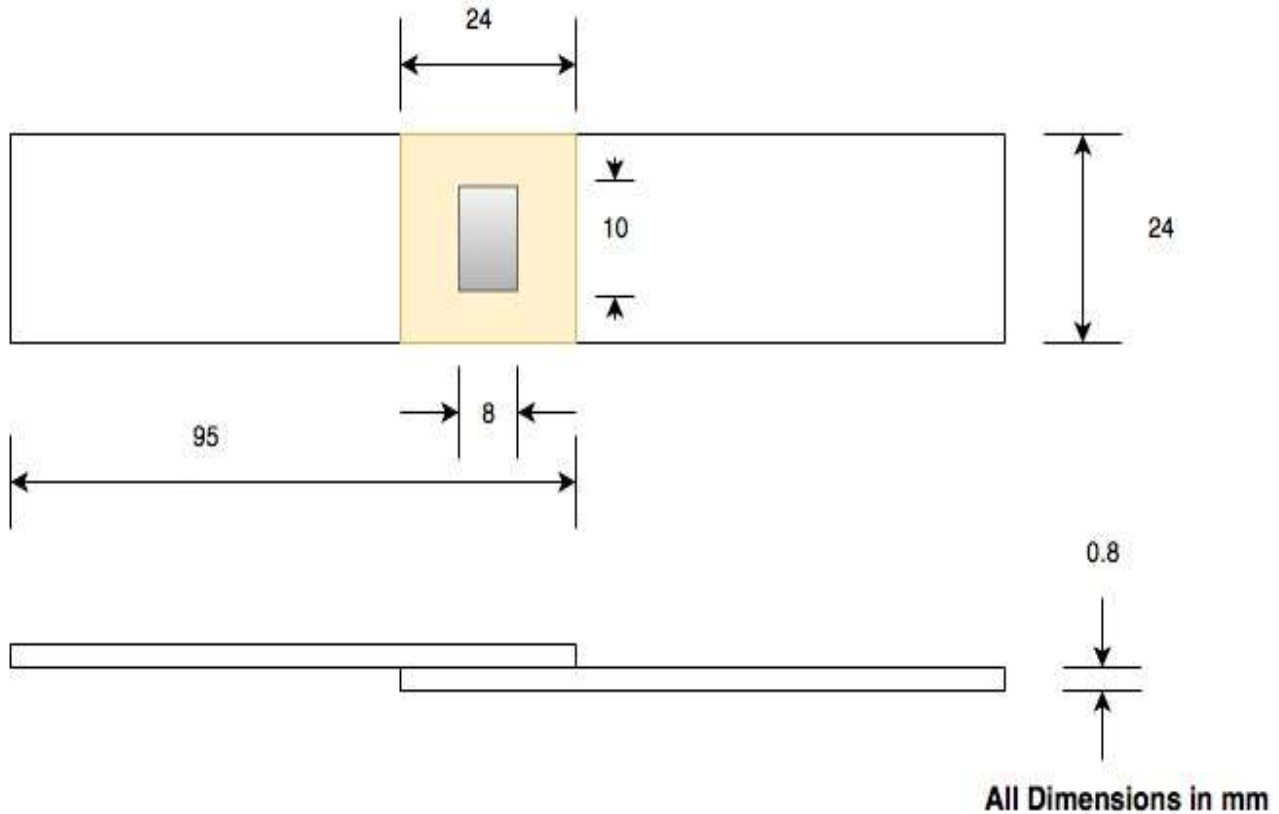
Fig. 2.1 specimen for ultrasonic welding
