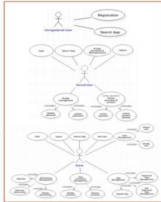
Figure (1) Use Case of SMEs-Portal
