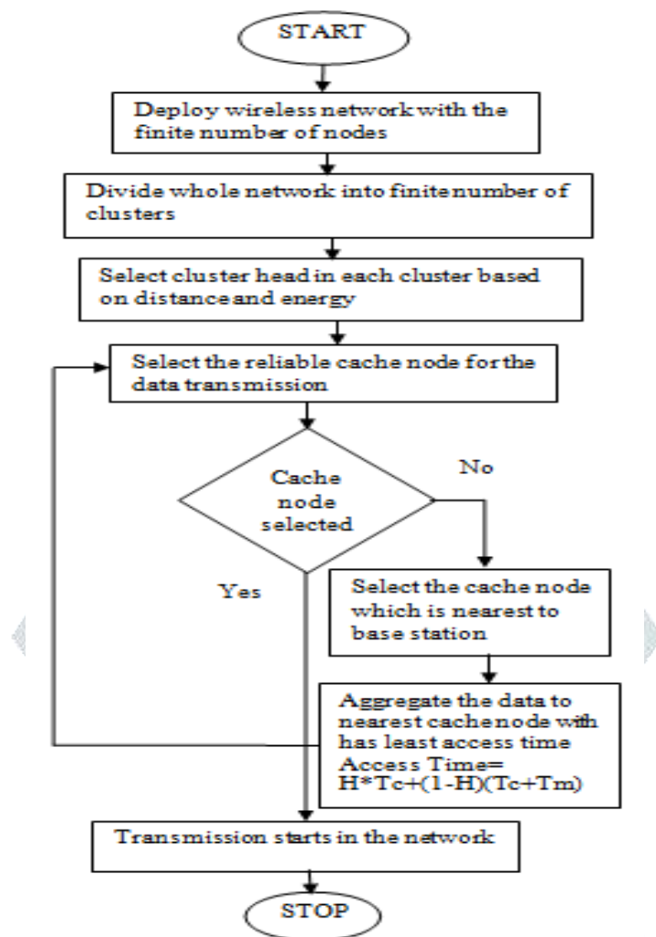
Fig 1: Selection of cache node
