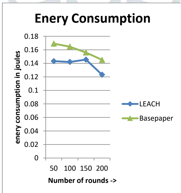
Fig 2: Energy Consumption
