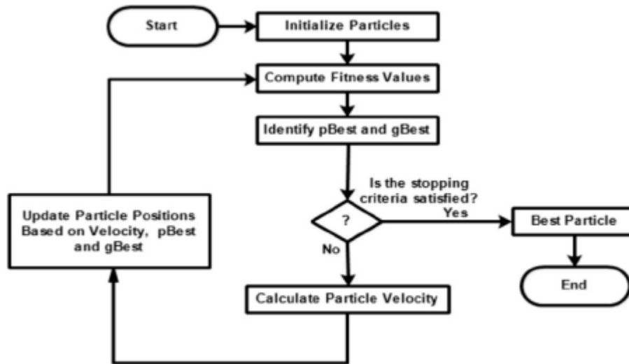
Flow diagram of PSO
