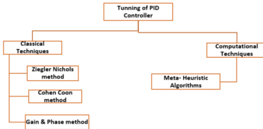
PID Controller Tuning Classification
