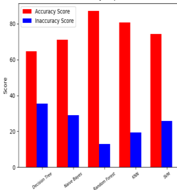
Figure 6 : Accuracy Graph
