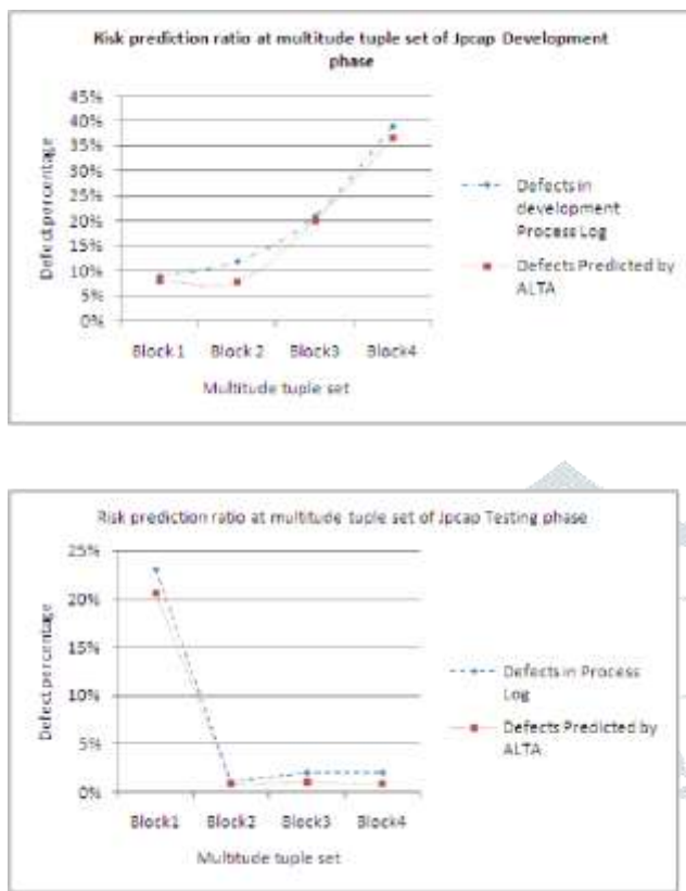
Fig 6: Line chart comparison of defects logged in process log and defects predicted by ALTA for mid size software development
