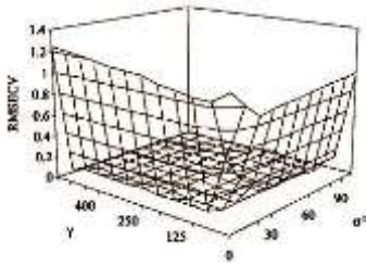
Fig 4: Hyper-Parameter optimization response surface under IWP-QPSO[29] for LS-SVM[25]
