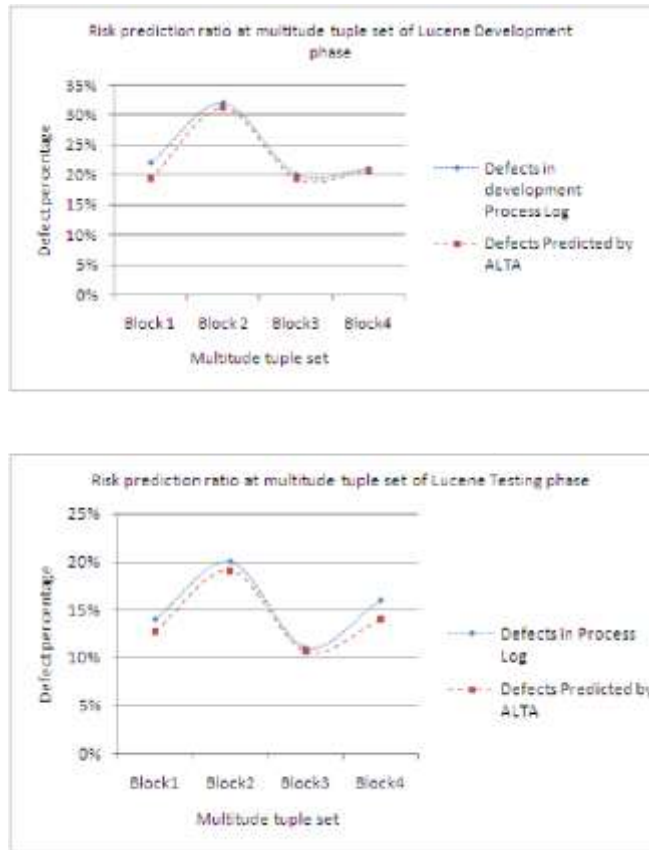
Fig 7: Line chart comparison of defects logged in process log and defects predicted by ALTA for large size software development
