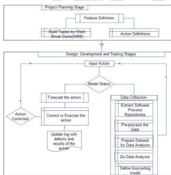
Fig 2: Defect prediction and handling using Machine learning
