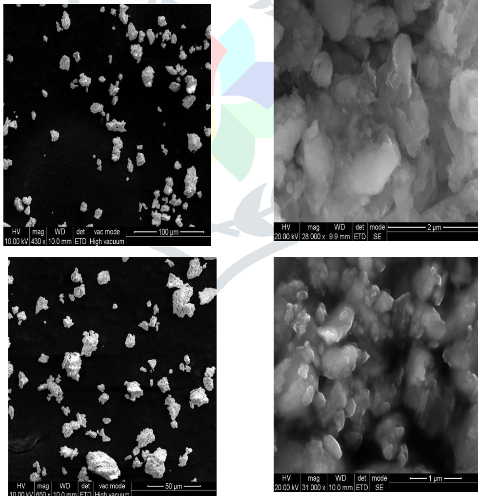
SEM Analysis of silver Nanoparticles
