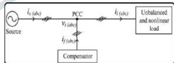
Fig.1. Proposed load compensation scheme
