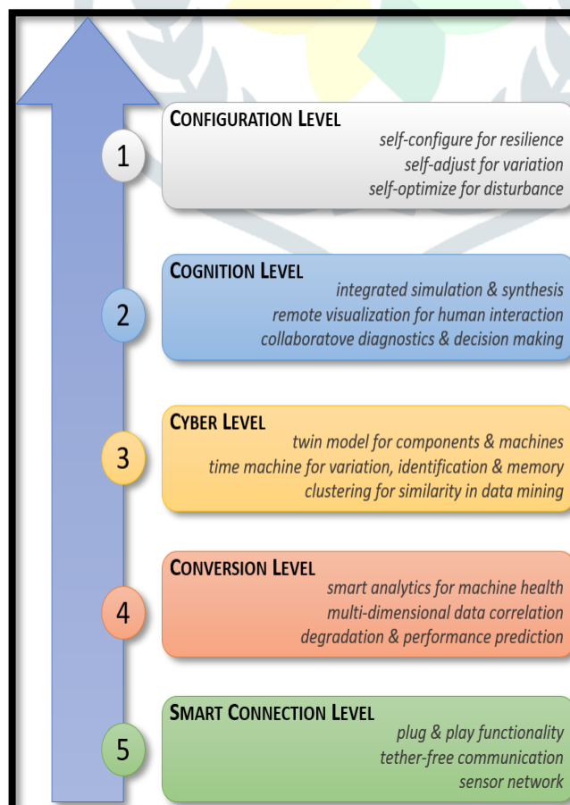
Figure 2. A Diagrammatic Presentation of CPS architecture
