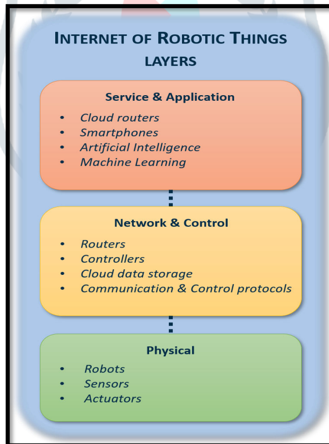
Figure 4:Internet of Robotics Things architectures Layers
