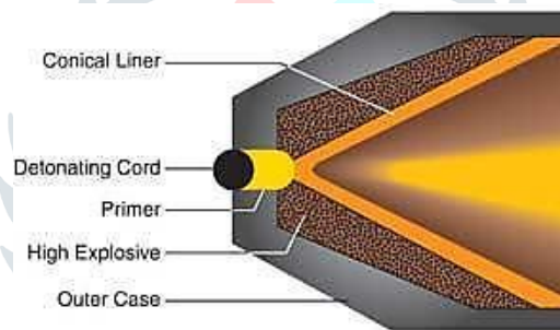
Figure 1: Schematic diagram of a shaped charge
