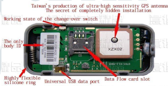
Fig. 3 Module- internal view
