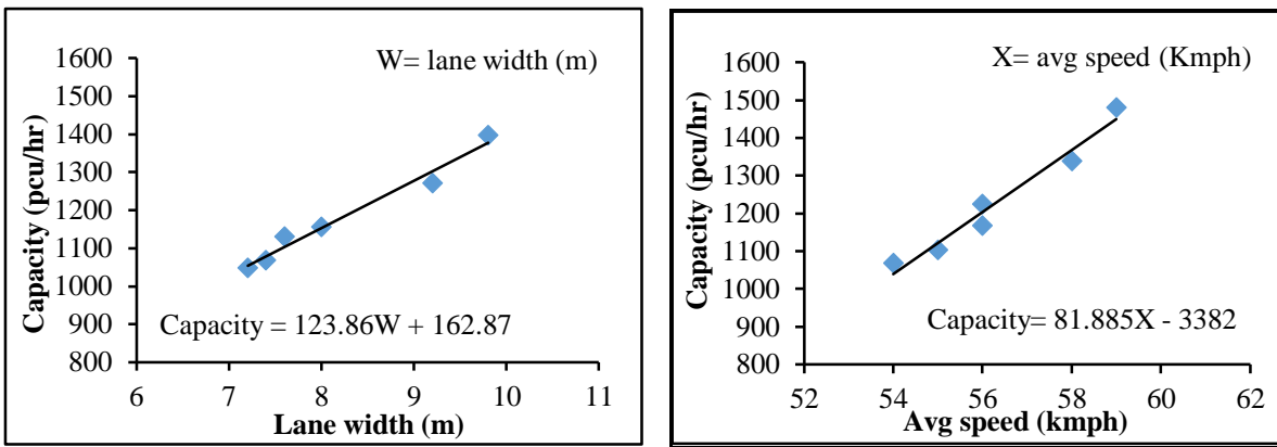
Fig-9 Capacity Vs Lane width and average speed at straight portion
