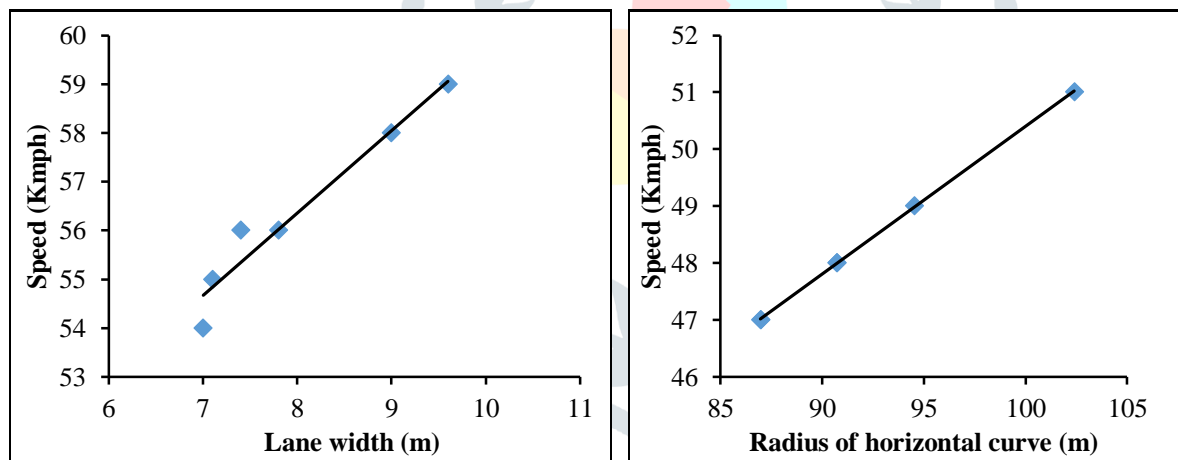
Fig-5 Speed Vs Lane width and Radius of horizontal curve
