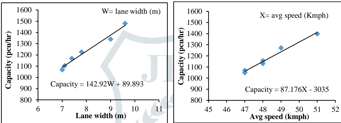
Fig-10 Capacity Vs Lane width and average speed at horizontal curve portion
