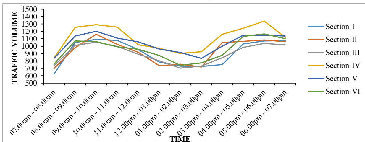
Fig-3 Hourly traffic volume variation at all sections
