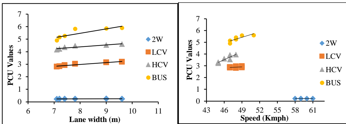
Fig-7 PCU values Vs Lane width and Speed at horizontal curve portion
