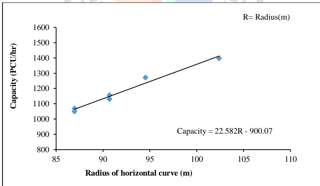
Fig-11 Capacity Vs Radius at horizontal curve portion
