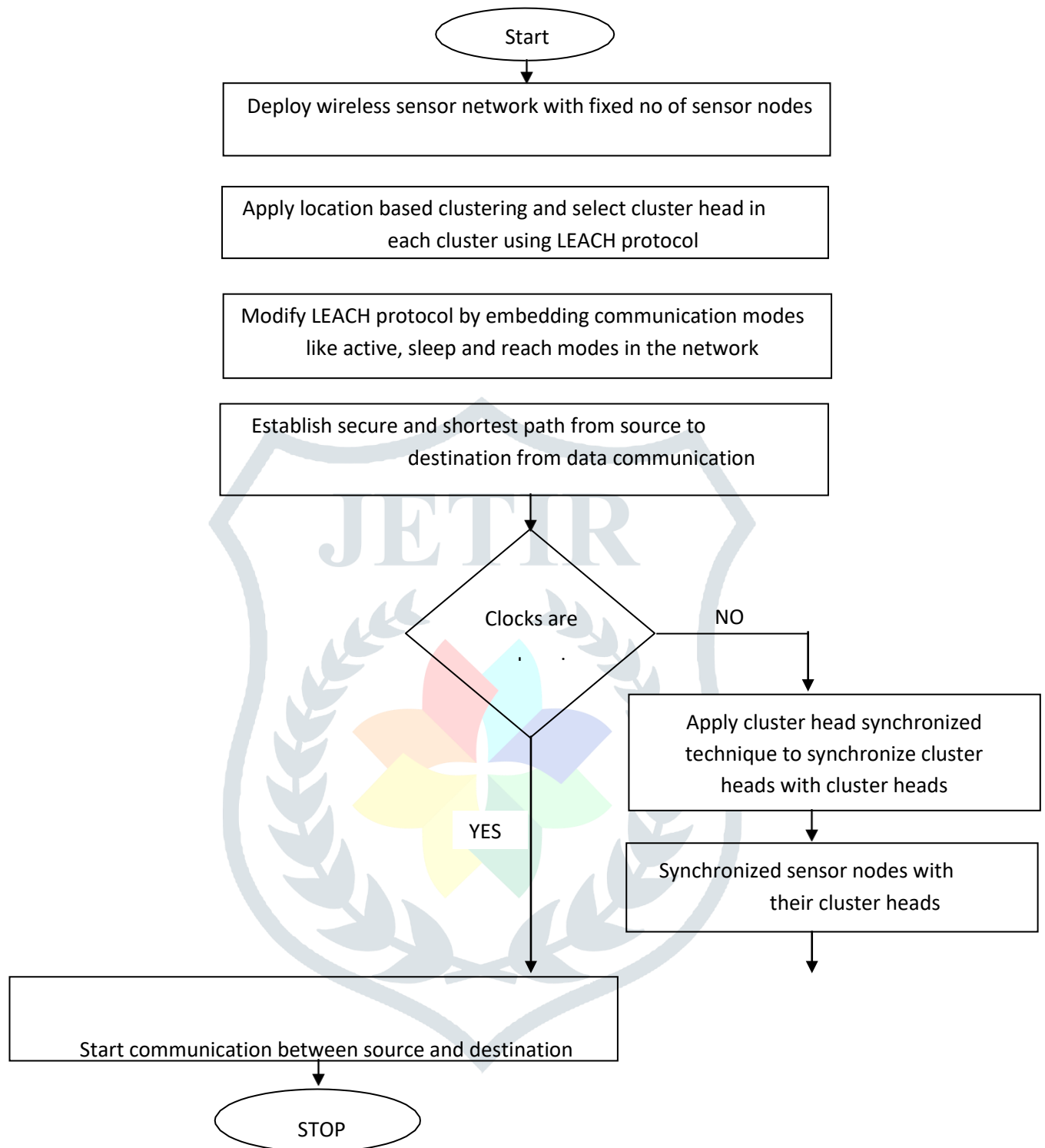
Figure 2: Proposed flowchart
