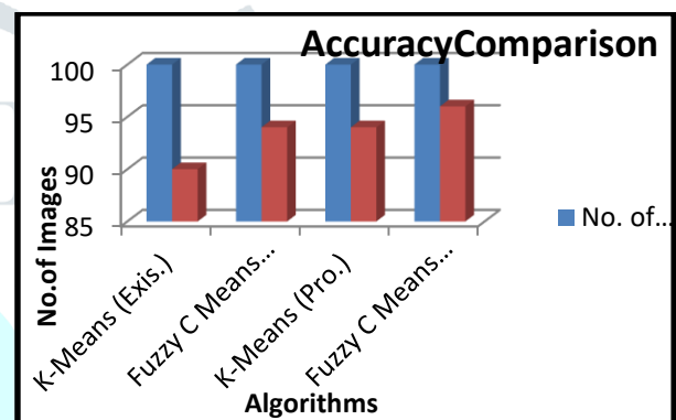
Fig. 7 Brain Image Clustering Accuracy Graph
