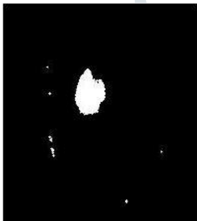
Fig. 5 Thresholding Segmentation
