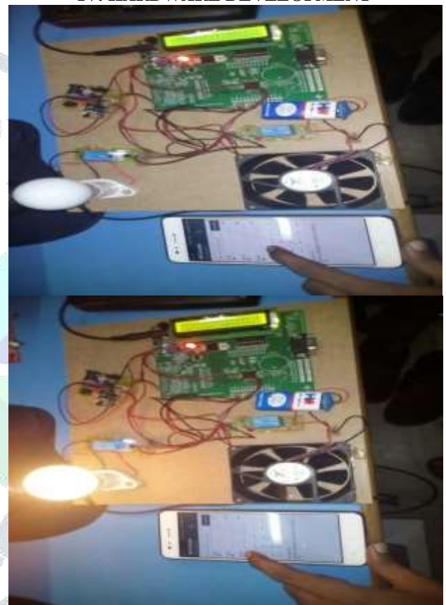
Figure13. Hardware Implementation.
