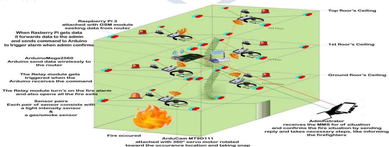
Fig. 2. System overview considering a three-storied building.
