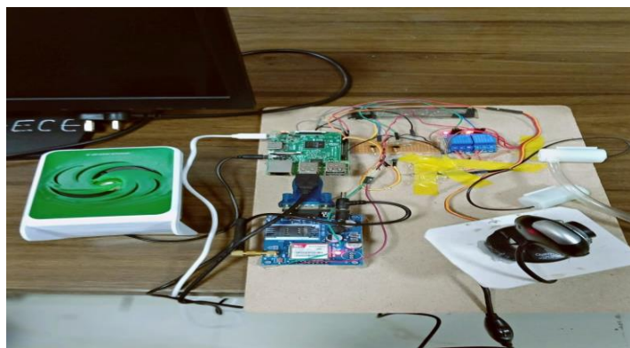
Fig. 5. Initial setup of proposed system
