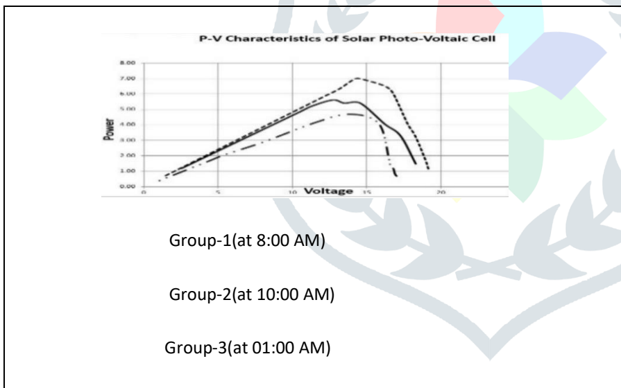
Fig.10 PV characteristic
