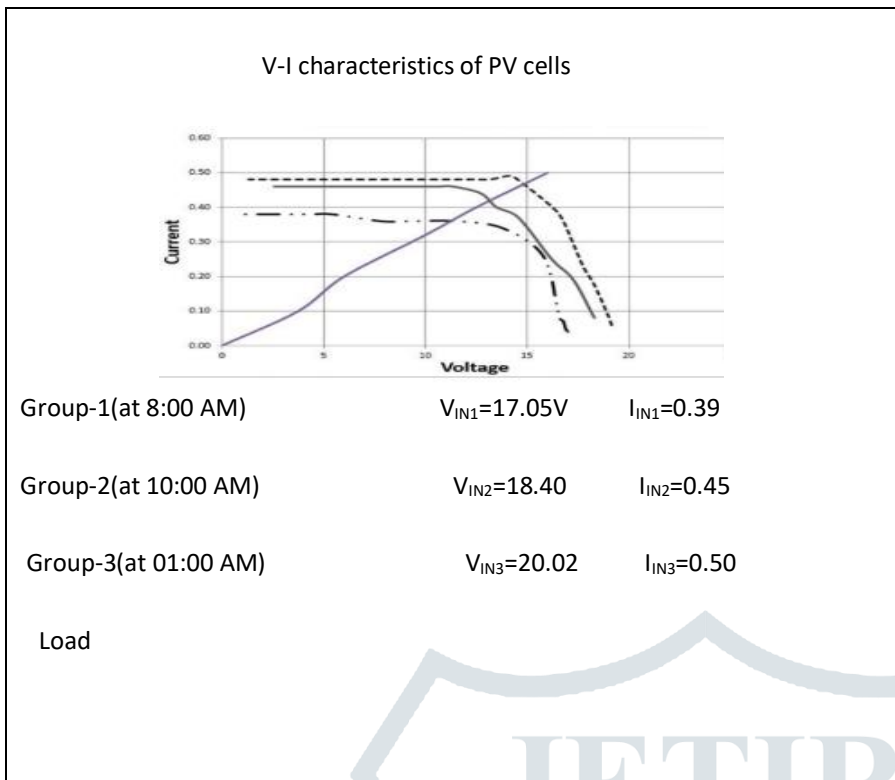
Fig.9 I-V and load characteristics of PV
