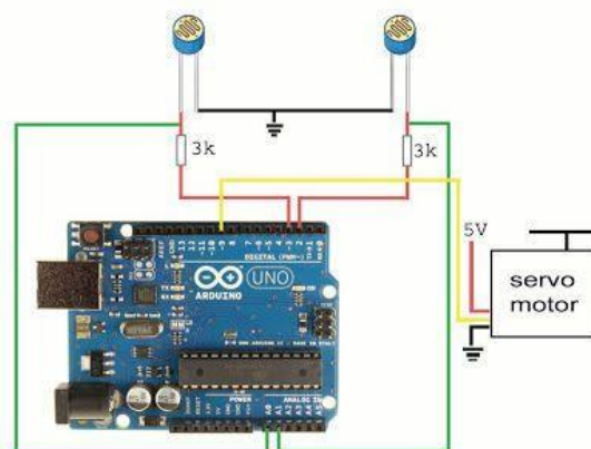
Fig.4 connection of Arduino Uno
