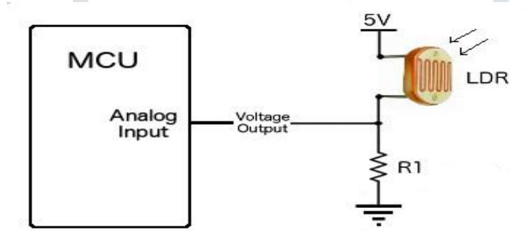
fig.5 the circuit diagram of LDR
