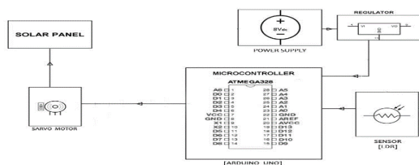
Fig.8 the complete diagram of MPPT
