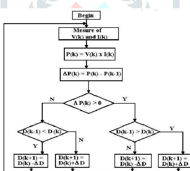
Fig.7the algorithm of P&O
