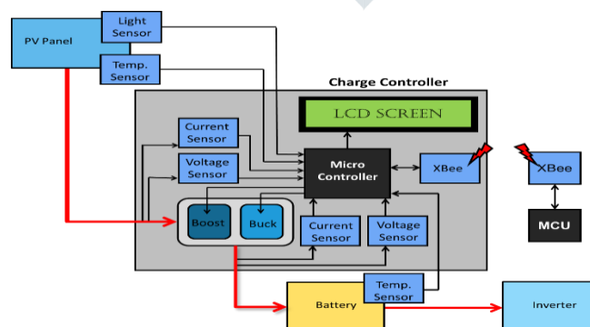
Fig.6 block diagram
