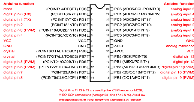
ATMega328P and Arduino Uno Pin Mapping
