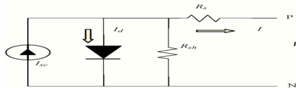
Fig.2 Equivalent circuit of solar PV
