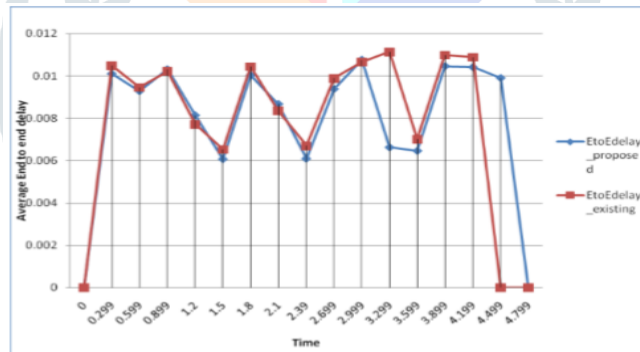
Fig7:Graph for End to End delay
