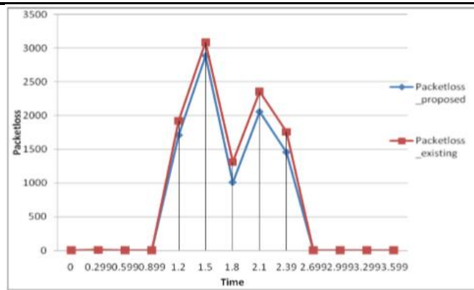
Fig 5: Graph of packet loss
