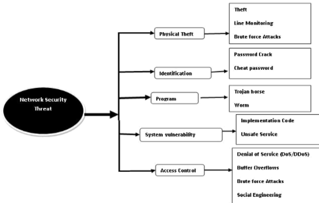
Fig. 1. Classification of Network Security Threats
