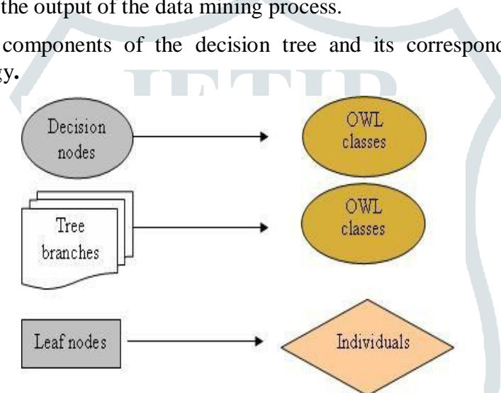
Figure 3 mapping decision tree to OWL ontology
