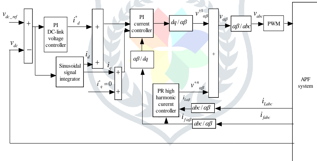
Fig.4 Model of DC link voltage control method.
