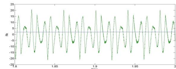
Fig. 11 Compensating current.
