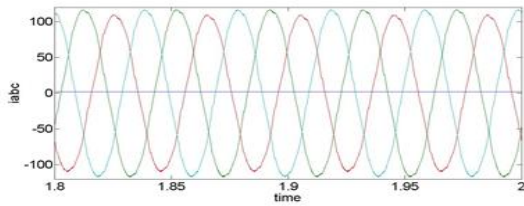
Fig. 13 Line current.
