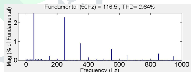
Fig. 12 (a) THD of line current
