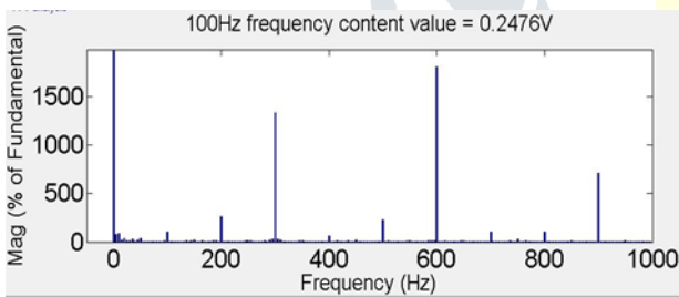
Fig. 16 (b) Harmonic content of DC link voltage.
