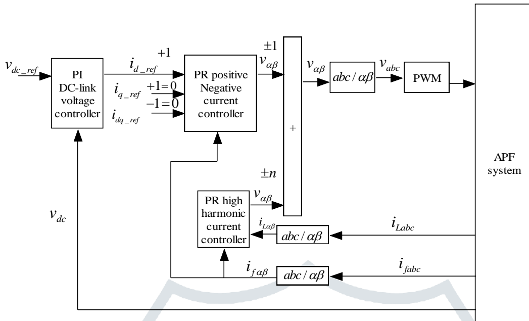
Fig.3 Model of Proposed PR control method.
